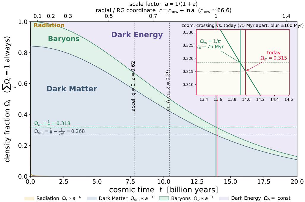
Figure 2: The cosmic energy budget through history, shown twice — the story of this paper in one image. Only the matter:vacuum seam moves; the \pi -locked inventory is the snapshot at the \Omega_m = 1/\pi crossing. Derived, and defended, in Part IV (Figure 22).
