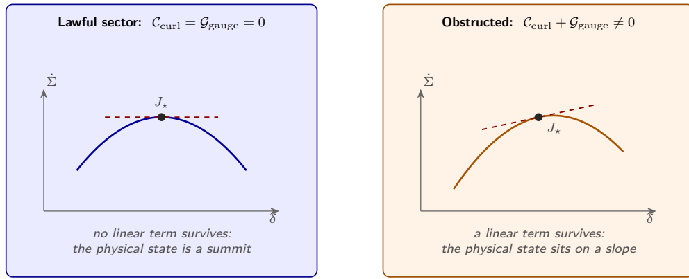
Figure 9: The mechanism of Theorem 30.1, drawn. Both panels plot the entropy production \dot{\Sigma} against an admissible variation \delta about the physical stationary current J_* of Eq. (30.1); the curvature is the same in both, because it comes from the same positive-definite inverse mobility. On the left the curl and gauge sectors do no work against the ledger, the cross term of the reduction vanishes, and J_* sits at the summit — which is what makes the flux-side and force-side readings of Theorem 28.2 extremal characterizations at all. On the right one of those sectors does work, a term linear in \delta survives at J_* , and the same curve is tilted: the dashed tangent no longer lies flat, and a point with a surviving linear term sits on a slope rather than on a summit. The tilt is not qualitative — it is -(C_{\text{curl}} + G_{\text{gauge}})/\Theta_{\text{eff}} , so the work the two sectors do against the ledger is the slope, and no functional of the entropy-production family is stationary where that work is nonzero. Read the two panels as one statement: the extremum readings are not approximately true outside the lawful sector, they are structurally absent there.
