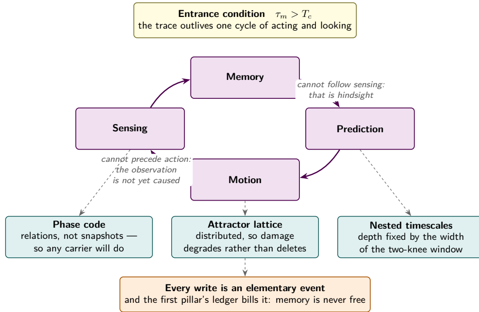
Figure 12: The architecture a system falls into once it keeps a trace for longer than a single cycle of acting and looking — the entrance condition at the top, which is a comparison of two times and nothing more. The loop’s order is not a modeling choice: sensing cannot come before action without the system knowing an observation it has not yet caused, and prediction cannot come after sensing without becoming hindsight, so each rearrangement destroys a step that has work to do. Three motifs hang off the loop. What is stored is a set of relations between phases rather than the phases themselves, which is why the same content survives being carried on a completely different rhythm and why a chemical, a neural and a digital system can hold it on unrelated hardware. The store is a lattice rather than a filing cabinet, which is why damage degrades a memory instead of deleting a list. And the ladder of nested timescales is only as deep as the spectral window of the preceding Part allows. At the foot: a write is an elementary boundary event, so the ledger of the first pillar prices it. What is established is a canonical normal form rather than a proof that no other shape could exist.
