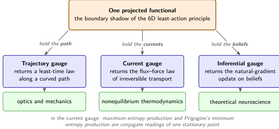
Figure 8: How three principles that look like rivals turn out to be one. The single projected functional at the top is the boundary image of the six-dimensional least-action principle; it is not a new postulate. Each arrow is the same stationarity condition asked with a different quantity held primary, and the label on the arrow names which: hold the path and the condition returns a least-time law, hold the currents and it returns the flux-force relation of irreversible transport, hold the beliefs and it returns the natural-gradient update used in the brain sciences. The bottom row names the community that has been using each form. The dashed link records what the unification settles on the way through: maximum entropy production and Prigogine’s minimum entropy production are conjugate readings of one stationary point under dual control conventions — the first fixing the transport law, the second the state — not competing claims about nature. One system may occupy all three gauges at once — a cell following a gradient traces a path, maintains fluxes, and corrects an estimate.
