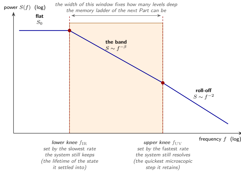
Figure 11: The claim that makes this pillar falsifiable. Systems of this kind are known to show 1/f noise, and that observation on its own is worth very little, because an unbounded power law is compatible with a great many mechanisms and so eliminates almost none of them. What is predicted here is a bounded band: the spectrum is flat below the lower knee, follows a power law between the knees, and steepens to f^{-2} above the upper one. The two knees are not fitted. The lower sits at the slowest rate the system still keeps — the lifetime of the state it settled into — and the upper at the fastest it still resolves, so a measurement can disagree with either independently. The exponent in the band, the heaviness of the jump distribution, and the dimension of the set the system explores are all controlled by one number, so those are one claim rather than three pieces of evidence. Where the paper places known observations from other fields against this shape, they are placements: a retrodiction of 1/f noise is nowhere treated as a confirmation.
