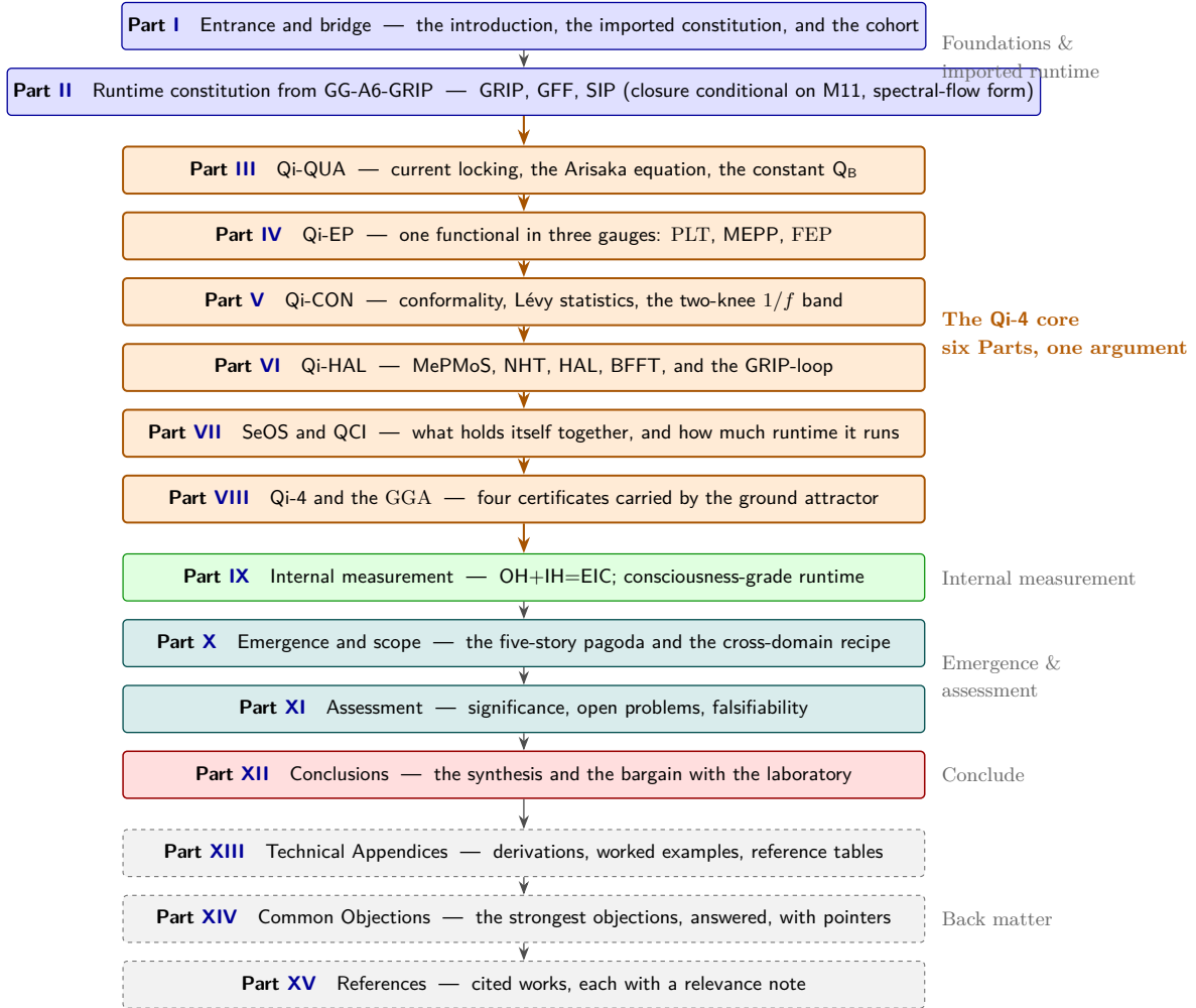
Figure 3: Roadmap of the fifteen Parts of GG-A7-Qi4. The argument develops in five phases. Foundations and the imported runtime (Parts I–II): the entrance and bridge, then the runtime constitution GRIP, GFF, and SIP imported from GG-A6-GRIP, whose closure is conditional on that companion’s remaining cascade conditioning — the monodromy statement M11 in spectral-flow form, with the budget question M10 resolved externally and the scope refinements closed at class level by the three-generations companion. The Qi-4 core (Parts III–VIII), the six banded Parts: the four informational pillars established as principal theorems in their dependency order ( Qi-QUA \Rightarrow Qi-EP \Rightarrow Qi-CON \Rightarrow Qi-HAL ), then the persistence and completeness layer (SeOS, QCI), then the statement that the ground attractor of the geometric companion carries all four pillar certificates — proved in that direction, with the converse recorded as open. They are drawn as one block because they are one argument told in six instalments, and the block is highlighted because it is the paper’s central claim. Internal measurement (Part IX) builds the outer and inner holograms and the loop that couples them on top of the pillars. Emergence and assessment (Parts X–XI): the five-story pagoda and the cross-domain recipe, then significance, open problems, and falsifiability. The conclusions (Part XII) close the argument, and the three back-matter Parts collect the technical appendices (Part XIII), the common objections and responses (Part XIV), and the annotated references (Part XV).
