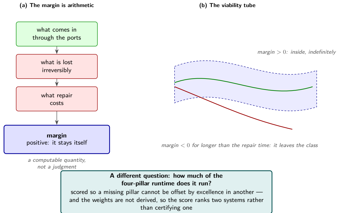
Figure 13: Two questions this Part separates, which are usually asked as one. (a) Whether a thing can hold itself together is arithmetic: what comes in through the ports, minus what is irreversibly lost, minus what repair costs. The margin is a computable quantity rather than a judgment, and it can be evaluated for a protocell, a reef, or an institution. (b) Averaged over a window longer than the system’s own repair time, a positive margin keeps the trajectory inside the region where the system is still itself; a margin that stays negative for longer than that carries it out, and it stops being a member of the class. The lower band asks something different and only loosely correlated: how much of the four-pillar runtime the surviving system actually runs. That score is built so that a system missing one pillar cannot compensate with excellence in another, because that is what incompleteness means — and its weights are not derived, so the honest use of it is to rank two systems and not to certify one. The persistence class is defined against the survival of a particular packet and carries no suggestion of intention or of moral standing.
