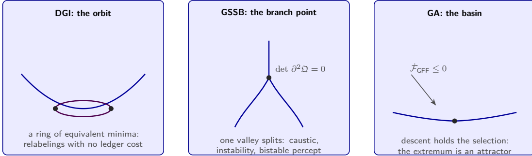
Figure 10: The three moves of the runtime engine acting on the Qi-EP landscape, drawn one per panel. Left, DGI: gauge transformations carry no ledger cost, so a stationary point is a ring of equivalent minima and the physical content lives on the orbit space — in the inferential gauge this is exactly why the natural gradient, and not the naive one, appears in Eq. (29.8). Center, GSSB: where the selector’s Hessian degenerates a valley splits, and the three gauges meet this single condition as the caustic of optics, the convective instability of the current reading, and the bistable percept of the inferential one — three literatures’ edge cases as one degeneracy. Right, GA: in the gradient sectors the ledger descends monotonically, so what the selector picks the runtime keeps; the basin’s depth is the quantity Part VII converts into a persistence class. The figure is a schematic of mechanisms, not a computed surface, and each panel’s claim is carried by the theorem it cites in the text.
