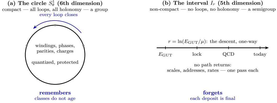
Figure 6: The anatomy of the two fibers. (a) The compact phase circle: every path closes, so everything a connection does there is holonomy — quantized (the dots are the ledger-rational marks), gauge-protected, transported by a group. (b) The scale interval: no path closes, so nothing is protected; transport composes only forward, a semigroup, and the descent visits each scale exactly once. This is why a stable bit is holonomy-class data on the circle while erasure is a one-way write along the interval, why Landauer’s bound prices only the second of those, and why the two audits are not competing bounds on one quantity. Carried from the holonomy white paper, where the anatomy is the subject rather than a tool.
