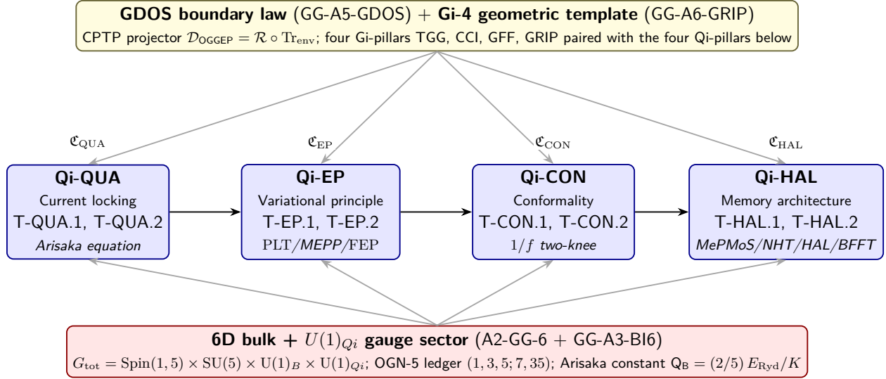
Figure 4: Architecture overview of the four Qi-4 pillars. Each pillar inherits its constitutional content from the GDOS boundary law of A5 paired with the Gi-4 geometric template of A6 (top), and its bulk-side technical content from the 6D bulk + U(1)_{Q_i} gauge sector (bottom). Horizontal arrows show the implication chain \text{Qi-QUA} \Rightarrow \text{Qi-EP} \Rightarrow \text{Qi-CON} \Rightarrow \text{Qi-HAL} . The four named compatibility propositions \mathcal{C}_{\text{QUA}}, \mathcal{C}_{\text{EP}}, \mathcal{C}_{\text{CON}}, \mathcal{C}_{\text{HAL}} (one per pillar) tie the algebraic (T-*.1) and operational (T-*.2) layers within each pillar.
