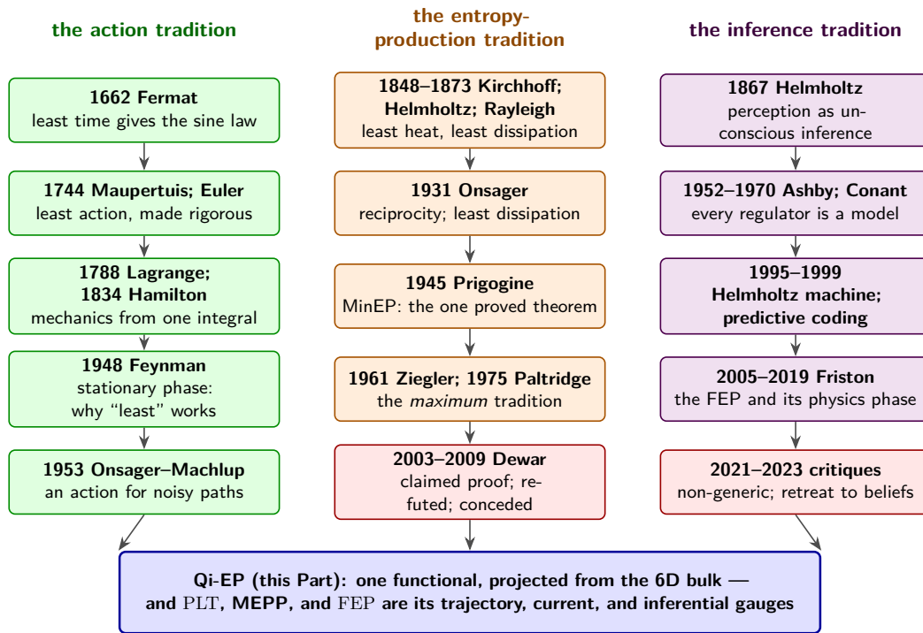
Figure 7: The genealogy of the three extremal principles, drawn as three columns that never cite one another. Left, the action tradition: from Fermat’s least time through Maupertuis, Euler, Lagrange, and Hamilton to Feynman’s stationary phase and the Onsager–Machlup stochastic action. Center, the entropy-production tradition: from the least-heat and least-dissipation theorems of Kirchhoff, Helmholtz, and Rayleigh through Onsager and Prigogine to Ziegler’s maximum, Paltridge’s climates, and the claimed general derivation that was refuted and conceded. Right, the inference tradition: from Helmholtz’s unconscious inference through cybernetic regulation and the Helmholtz machine to predictive coding, the free energy principle, its physics phase, and the critiques that forced its retreat. Each column ends unresolved in its own literature; the convergence at the foot — one projected functional whose three gauges they are — is the claim this Part derives, and the dates above it are why the derivation is worth having.
