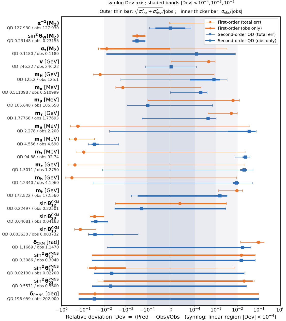
Figure 2: The full 28-parameter audit in one panel: all twenty-two directly benchmarked Standard-Model parameters on a symmetric-log deviation axis — first order (orange) and second-order QD (blue) against measurement, nested precision bands at 10^{-4}, 10^{-3}, 10^{-2} . Full version: Figure 9 in Part II.
