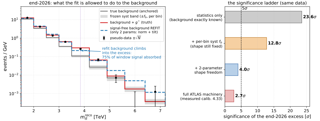
Figure 11: Why the “clean” excess of Figure 12 is worth 2.5–2.7 \sigma , not 20 \sigma , at end-2026. Left: the end-2026 spectrum with the frozen per-bin systematic band (gray) and the signal-free background refit with only two free parameters, normalization and tilt (blue dashed): the refit climbs into the excess and absorbs 75% of the window signal, at negligible cost at low mass where the band is tight. The full ATLAS fit has \mathcal{O}(100) such degrees of freedom. Right: the significance ladder of the identical dataset: perfect-background counting 23.6 \sigma \rightarrow per-bin systematics 12.8 \sigma \rightarrow two-parameter shape freedom 4.0 \sigma \rightarrow measured full-analysis calibration 2.7 \sigma .
