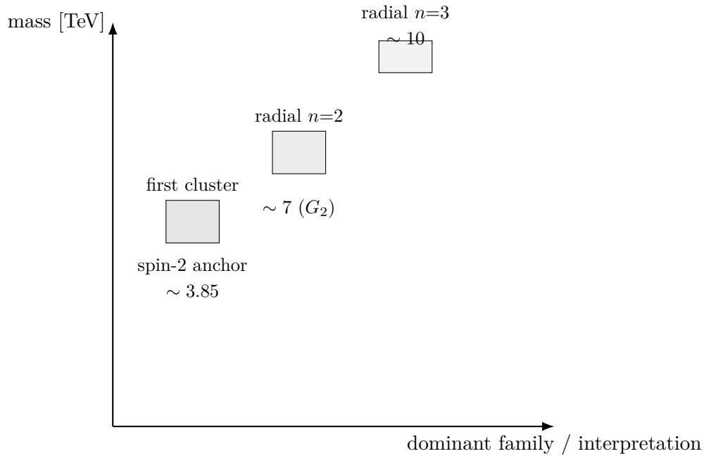
Figure 5: Schematic mass staircase of the low-lying GG-6 sector. The figure is not a claim of exact line positions beyond the first centroid. It is a search map: the lock-scale cluster — a Neumann octet g^* , a Dirichlet baryonic vector Z'_B , and the spin-2 graviton, all at \approx M_{\text{lock}} \approx 3.85 TeV up to O(1) coefficients — and the next radial families near 7 TeV ( n = 2 ) and 10 TeV ( n = 3 ). The angular partners, if they propagate, sit at derived offsets just above the cluster (Eq. (12)) and are absent from single production.
