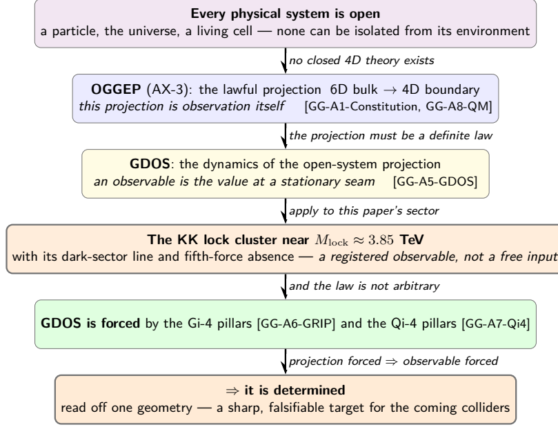
Figure 1: The central claim, as one deductive funnel, shared across the GG-Theory cohort. Because no physical system is closed, the four-dimensional world is a lawful projection (OGGEP, AX-3) of the six-dimensional bulk, and that projection is observation itself; its dynamics is GDOS, forced by the Gi-4 and Qi-4 pillars. The same funnel opens the companion papers GG-A9-SM, GG-A10-Cosmos, and GG-A11-Origin; only the payload differs — here, the Kaluza–Klein lock cluster.
