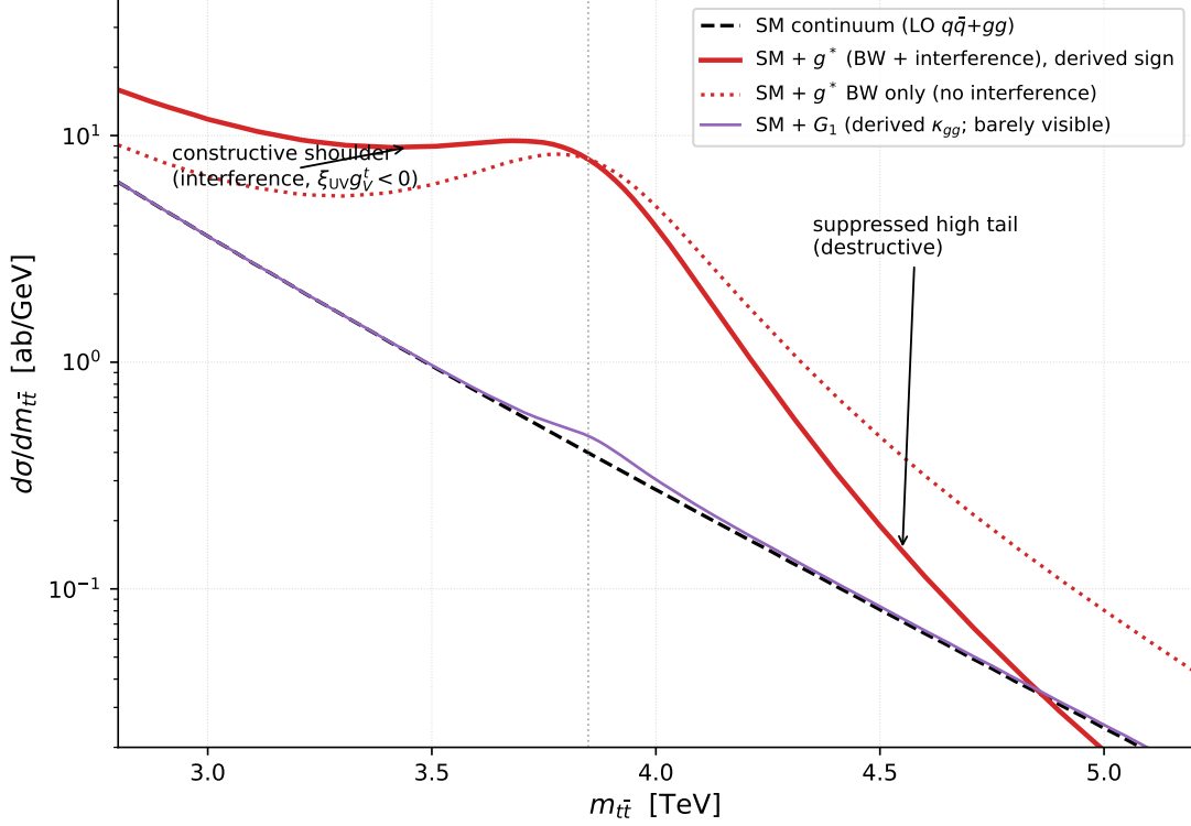
Figure 6: The LO m_{t\bar{t}} spectrum near the lock scale at \sqrt{s} = 13 TeV. Red solid: SM + g^* with the full interference of Eq. (66) at the derived sign \xi_{UV} g_V^t < 0 ; red dotted: Breit–Wigner only. The constructive low-side shoulder, the destructive collapse of the high tail (crossing below the SM at \simeq 4.9 TeV), and the near-invisibility of G_1 (violet) are the three structural signatures. Numbers in Table 14.
