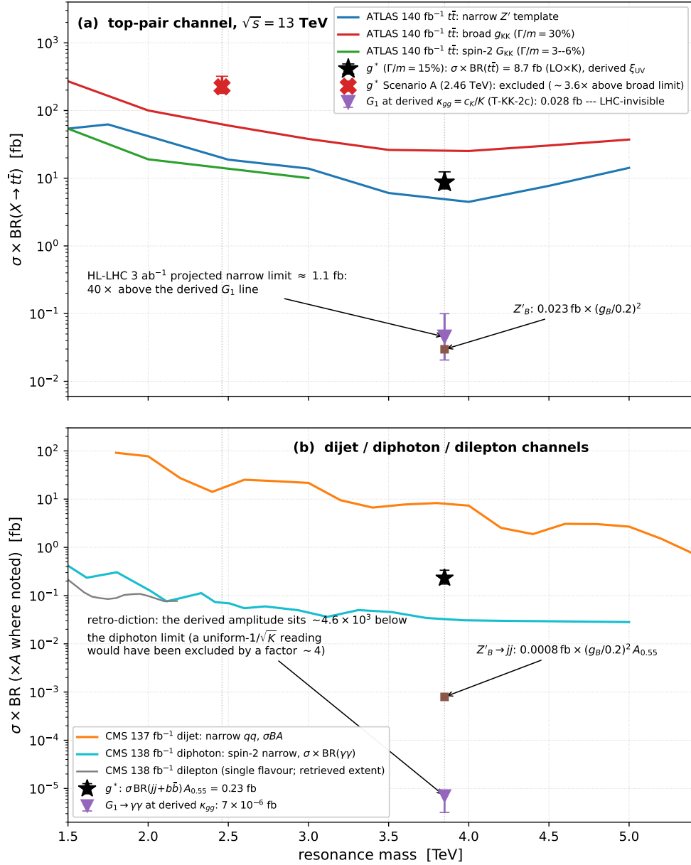
Figure 9: The operational confrontation at \sqrt{s} = 13 TeV, all couplings at their derived values (T-KK-2, T-KK-2c). Panel (a): observed 95% CL limits from the ATLAS 140 fb ^{-1} t\bar{t} -resonance search (ATLAS Collaboration, 2025a) (narrow- Z' , broad-KK-gluon \Gamma/m = 30\% , and spin-2 templates; HEPData ins3094414) against the predictions of Table 19: the Scenario-B octet at 8.7 fb (star) — the un-suppressible line that carries the HL-LHC falsifier; the Scenario-A octet at 2.46 TeV (red cross), a factor \sim 3.4 above the observed broad-template limit on the window content and 19 on the peak-region transfer (F-KK-2A fired); and G_1 at the derived \kappa_{gg} = c_K/K (violet triangle, 0.045 fb) — a factor \sim 25 below even the 3 ab ^{-1} HL-LHC projection, hence LHC-invisible. Panel (b): the CMS narrow-dijet \sigma BA limit (CMS Collaboration, 2020b), diphoton spin-2 limit (CMS Collaboration, 2024a), and dilepton limit over its retrieved extent (CMS Collaboration, 2020), against the octet dijet rate ( \sigma BA = 0.30 [0.23–0.43] fb), the Z'_B 's Neumann reference as a withdrawn upper bound, and G_1 \rightarrow \gamma\gamma at the derived coupling ( 1.1 \times 10^{-5} fb): the published diphoton null is retro-dicted with a margin of \sim 3 \times 10^3 , whereas a uniform- 1/\sqrt{K} photon amplitude would already be excluded by a factor \sim 4 . All predictions LO \times K with stated bands, at the values of Table 19.
