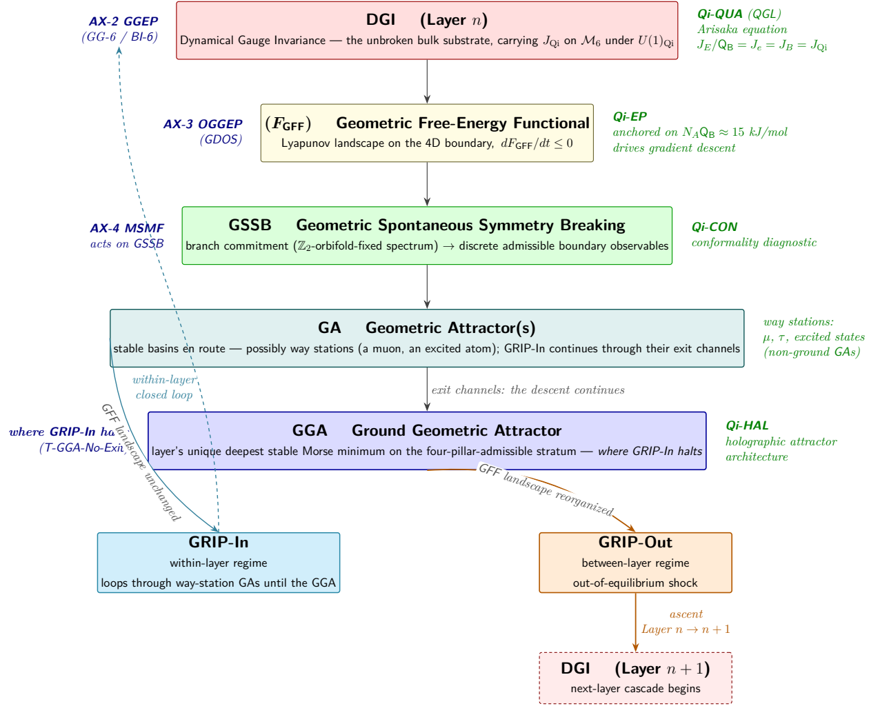
Figure 8: The GRIP engine: four moves, two regimes, one ground state. The central column is the four-move descent \text{DGI} \rightarrow (F_{\text{GFF}}) \rightarrow \text{GSSB} \rightarrow \text{attractor} ; the three constitutional axioms (left) force the moves and the four Qi-4 pillars (right) filter the Morse minima. GRIP-In (cyan) loops within a layer to the unique ground state; GRIP-Out (orange) reorganizes the landscape and opens the next floor. The four pillar names on the right (Qi-QUA, Qi-EP, Qi-CON, Qi-HAL) and the minimality axiom MSMF on the left are stated in Chapter 15; nothing before that chapter uses them. The four moves are walked in order through the rest of this chapter (§§14.1–14.7).
