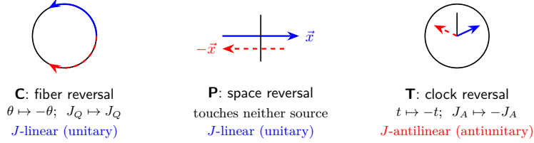
Figure 10: The three orientation reversals of T-P5-1. The fiber reversal flips the rotation generator and the signed charge together, leaving J_Q = \partial_\theta/Q invariant; the space reversal touches neither source of i ; the clock reversal is the one flip the imaginary unit is made of. The unitary/antiunitary table is the map of which reversals touch the sources. (after GG-P5-CPT)
