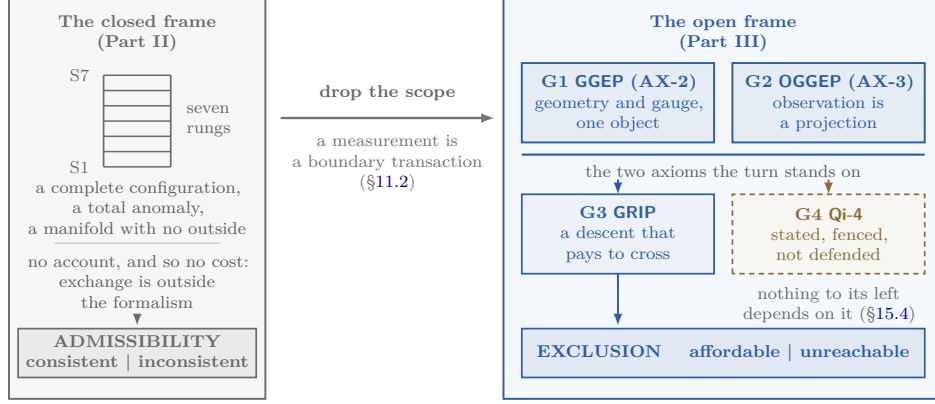
Figure 3: What the turn changes. The closed frame of Part II (left) reaches admissibility : its strongest tools — anomaly cancellation and integrality — sort candidate theories into consistent and inconsistent, and stop. They are silent about which consistent option obtains, because sorting by cost requires an account and an account requires a boundary. The open frame of Part III (right) is built on two axioms, carries a third move that stands on them, and a fourth that is stated and fenced; what it reaches is exclusion — not “inconsistent” but “unaffordable”. The whole of this Part is an argument that the step between the panels is forced rather than chosen, and Chapters 12–15 pay for it in assumptions, each named.
