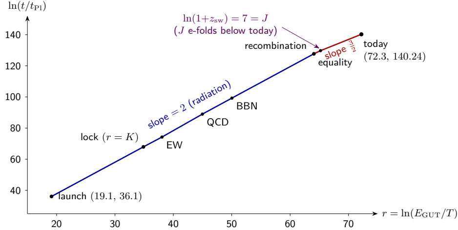
Figure 17: The whole history of time, on one line: boundary time (Planck units, logarithmic) against the radial coordinate (half-Planck convention), for eight epochs from the launch to today. The radiation era is a straight line of slope exactly 2 (89); the slope kinks to \frac{3}{2} at equality; the lock crossing sits at r = K = 35 ; the corridor switch sits J = 7 e-folds below today; the endpoint's audited decomposition is Eq. (90). Boundary time is the exponential shadow of the linear descent. (after GG-P5-CPT)
