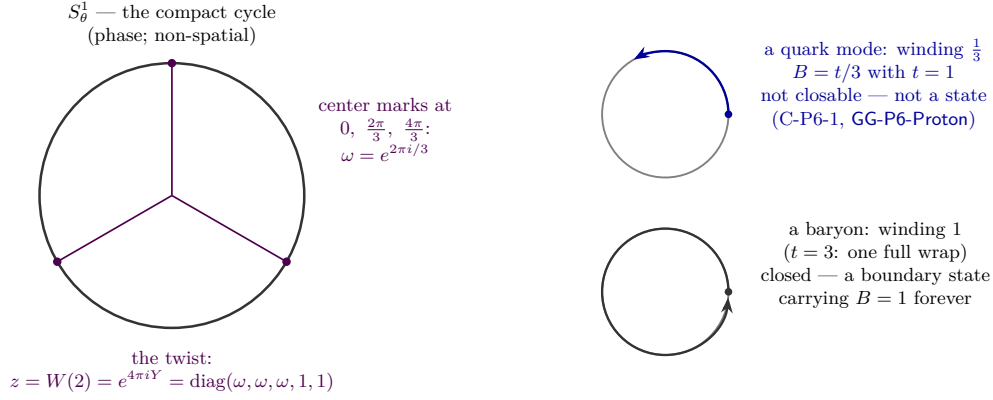
Figure 13: The color triangle — the lock, drawn. Left: the compact cycle S_\theta^1 with the twist at the unique center point of the hypercharge line — z = W(2) = e^{4\pi i Y} = \text{diag}(\omega, \omega, \omega, 1, 1) , the sole quantized holonomy passing the three-demand scan (GG-P6-Proton); its three marks at 0, \frac{2\pi}{3}, \frac{4\pi}{3} are the cube roots of unity — a three-fold lattice where the flavor sector had a five-fold one. Right: the two kinds of traveler. A quark mode winds by one third — an arc, not a loop: it cannot close, which is why no boundary readout ever carries it alone. A baryon winds once — a closed loop whose winding number is baryon number itself, B = t/3 by the center identity. A winding can no more be shed than a knot untied in a closed loop. One twist, four locks: the same third-of-a-turn breaks SU(5), lifts the X, Y , splits the Higgs, and writes e^{2\pi i B} = z — baryon number as the winding no operator can change (T-P6-2); that sentence, made precise, is the stability theorem. (after GG-P6-Proton)
