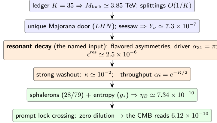
Figure 14: The leptogenesis chain as a flowchart: blue = inherited and derived, orange = the transport block carrying the named conjecture, green = standard reprocessing and conservation. The one direction of the whole diagram is the descent's. Every number is on the ledger; the one named input (the on-resonance condition) and the postulated exponent ( K/2 ) are stated in the text at their parent grades. (after GG-P5-CPT)
