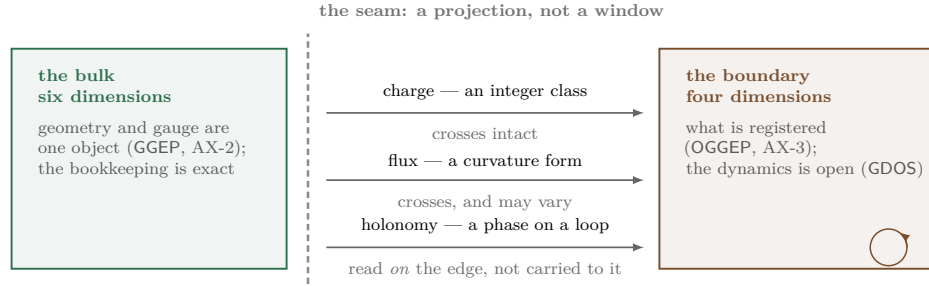
Figure 7: The seam. The three data of §10.2 crossing from a six-dimensional bulk to a four-dimensional boundary. The asymmetry is the point: the integer class crosses intact, the curvature form crosses and may vary, and the holonomy — being a statement about a loop — is evaluated on the boundary rather than transported to it. A closed theory can ignore the third row. An open one cannot (§13.4).
