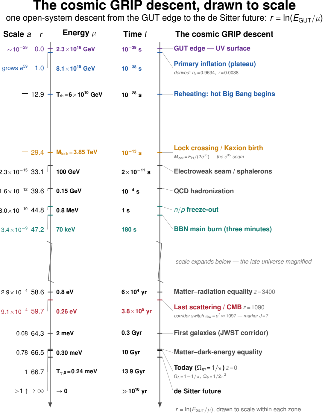
Figure 16: The cosmic GRIP descent, drawn to scale on r = \ln(E_{\text{GUT}}/\mu) . One open-system descent from the GUT edge ( r = 0 ) to the de Sitter future, read simultaneously in four quantities — energy \mu , time t , and the scale factor a , each against the radial depth r . The key epochs of the cohort’s master chronology (Arisaka, 2026, A10-Cosmos) are drawn to scale and colored, with the late universe magnified beneath the break so that recombination, structure, and the present epoch remain legible. Highlighted rows carry the framework’s derived markers: the plateau tilt and tensor ratio ( n_s = 0.9634 , r = 0.0038 ), the lock M_{\text{lock}} = E_{\text{Pl}}/(2e^{35}) = 3.85 TeV, the corridor switch z_{\text{sw}} = e^7 (integer-ledger marker J = 7 ), and today’s \pi -locked inventory ( \Omega_m, \Omega_\Lambda, \Omega_b ) = (1/\pi, 1 - 1/\pi, 1/2\pi^2) . Every value is a standard cosmological reading of that chronology; nothing on the axis is fitted.
