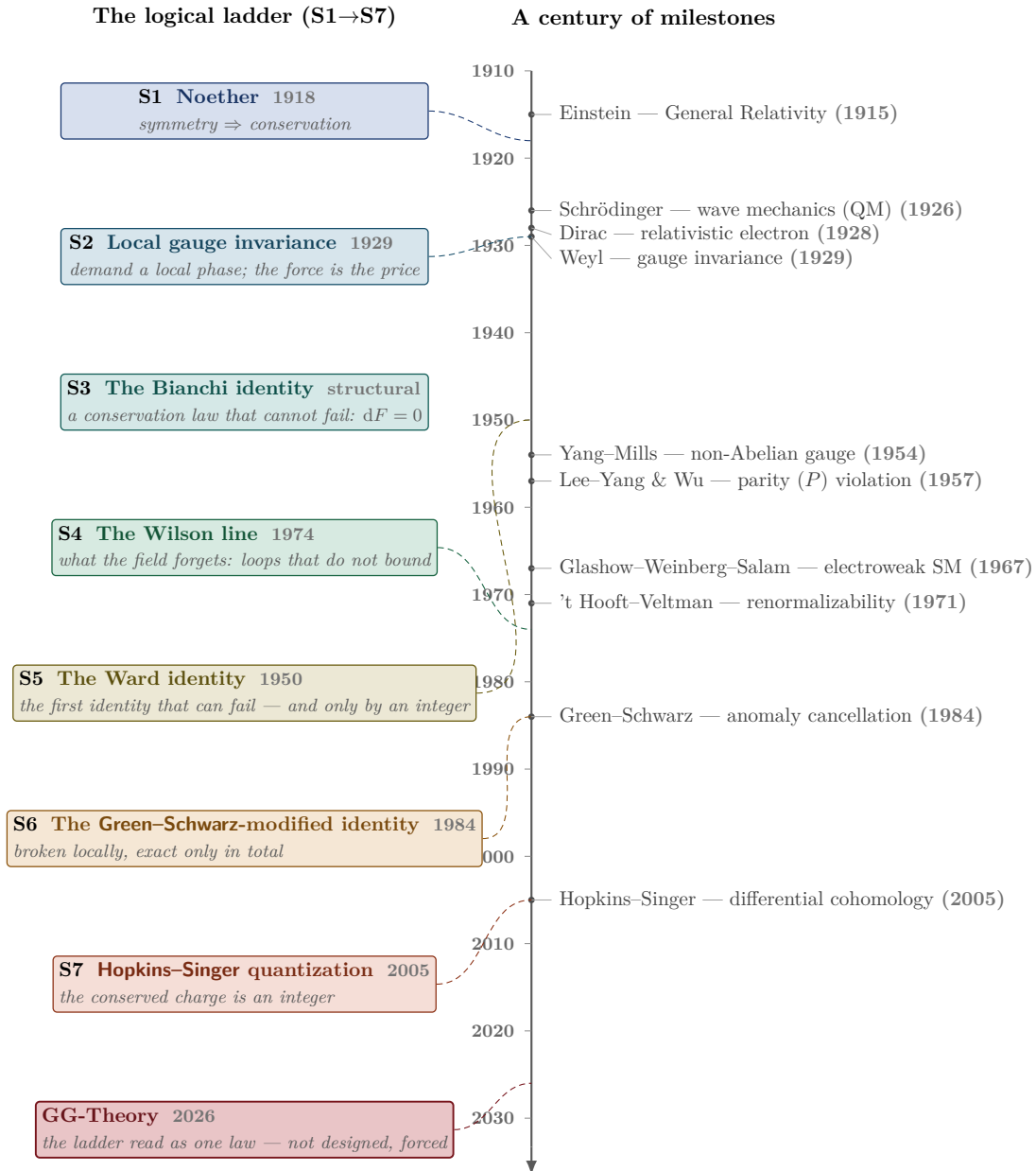
Figure 2: The ladder of Part II, set against real time. Left: the seven steps in their logical order — S1 at the top, GG-Theory at the foot — each tagged with the year of the idea it rests on. Right: a linear clock from 1910 to 2030 carrying the wider milestones the ladder draws on: general relativity, quantum mechanics, non-Abelian gauge theory, parity violation, the electroweak Standard Model, and more. Dashed lines join each dated rung to its year; they cross where the logical order departs from the historical one — the Ward identity (1950) sits logically after the Wilson line (1974), and the Green-Schwarz and Hopkins-Singer rungs rest on ideas that arrived only decades after Noether. The ladder is a reconstruction, not a chronology.
