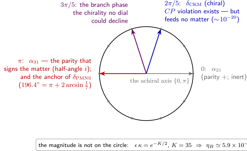
Figure 15: The alphabet audit, drawn: the ten letters of the pentagonal lattice on the one compact circle, with the four that decide the birth of matter marked. The quark Dirac phase (blue) is chiral but feeds no matter; the branch phase (violet) is the chirality the odd alphabet forced — the reason any interference exists to orient; the achiral letter \pi (red) does double duty as the Majorana parity that signs the matter and the anchor of the phase DUNE will measure; and the magnitude lives off the circle entirely, in the ledger’s throat depth. Existence from the pentagon, sign from a parity, size from the throat: three jobs, three structures, zero dials. (after GG-P5-CPT)
