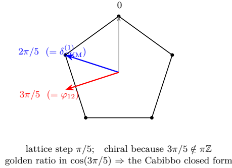
Figure 12: The flavor pentagon. With one compact circle and block integer L = 5 , first-order holonomies live on the lattice (\pi/5)\mathbb{Z} : the forced branch phase 3\pi/5 (red) is not a multiple of \pi , so CP violation must exist; one unphysical lattice step leaves the physical phase 2\pi/5 (blue); and the pentagon’s trigonometry — the golden ratio — sets the Cabibbo magnitude. One object, two of flavor physics’ deepest numbers. (after GG-P5-CPT)
