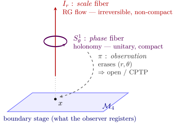
Figure 6: Observation as the bundle projection \pi : \mathcal{M}_6 \rightarrow \mathcal{M}_4 . Over each boundary point x sits the non-spatial fiber (I_r, S_\theta^1) . The compact phase circle S_\theta^1 carries the coherent, unitary content of quantum mechanics — its holonomy is the Aharonov–Bohm/Berry phase (Aharonov & Bohm, 1959; Berry, 1984) — while the non-compact scale interval I_r carries the irreversible, open content, its forward renormalization-group semigroup being the GKLS/GDOS generator. Because both fiber coordinates are non-spatial, no boundary protocol resolves them; every registration marginalizes the fiber, so \pi is non-invertible and the boundary dynamics is necessarily open. Unitary closure is the unreachable limit in which the fiber is not coarse-grained.
