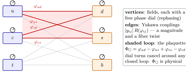
Figure 11: The flavor graph for three generations, drawn to the cohort’s wiring-diagram standard. Up-type and down-type fields are vertices, each carrying a freely re-settable phase dial; the nine Yukawa couplings are edges, each carrying a fiber twist \varphi_{ij} . Turning any dial shifts every edge at that vertex equally, so the shifts telescope to zero around a closed loop: the shaded four-edge plaquette holonomy \Phi_{\square} is invariant — a flavor-space Aharonov–Bohm phase (Aharonov & Bohm, 1959). For N = 3 , unitarity ties all such plaquettes to a single physical angle, the Jarlskog phase. (after GG-P5-CPT)
